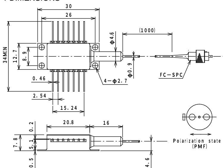
Package outline (Unit: mm)
